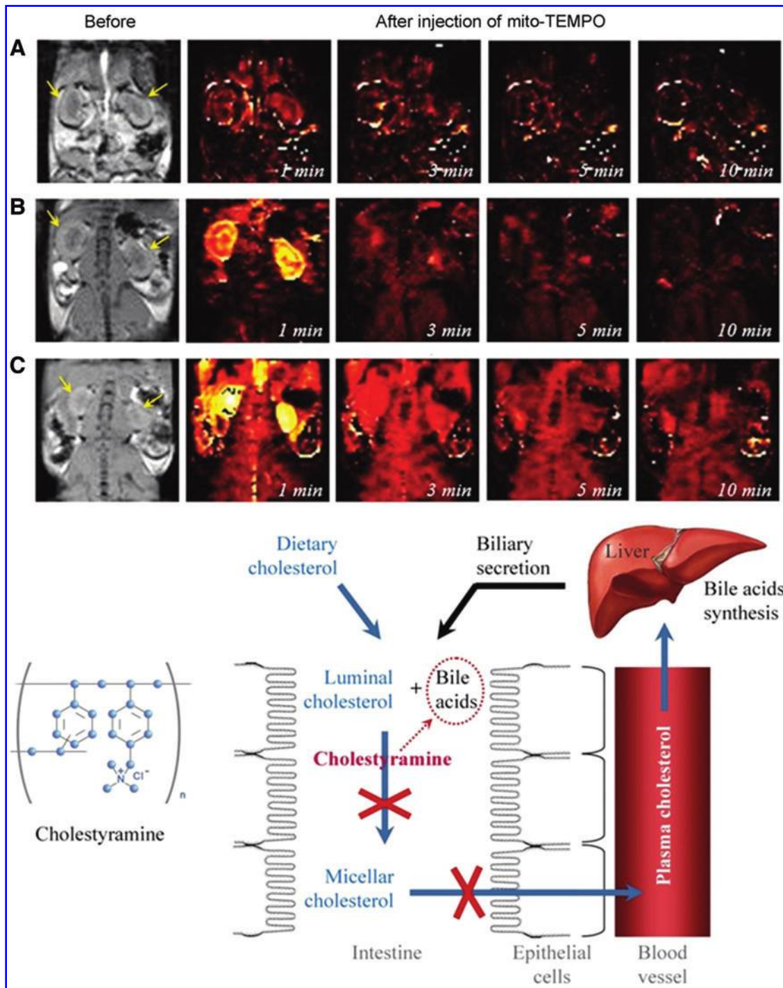
FIG. 19. Nitroxyl-enhanced MRI of the kidney in mice on a ND or high CD using mito-TEMPO as a contrast probe: black and white images: T 1 -weighted MR images of the kidney before the injection of mito-TEMPO. Color images: extracted MRI signal intensity normalized to the averaged baseline level (before the injection of mito-TEMPO): (A) ND; (B) cholesterol plus cholestyramine diet; (C) CD. The yellow arrows indicate the kidneys. Structural formula and mechanism of reduced plasma cholesterol by the bile acid sequestrant cholestyramine [according to Lazarova et al. (103)]. Color images are available online.
