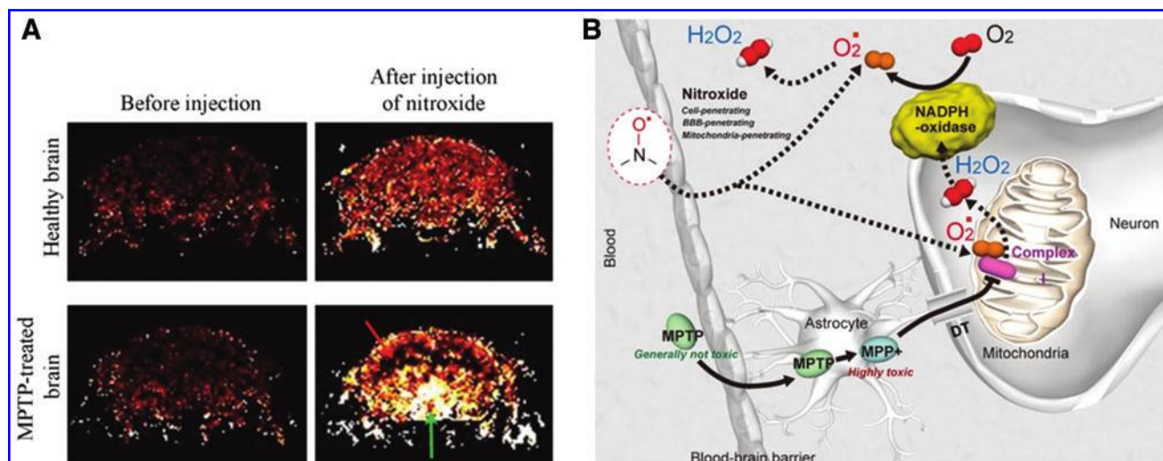
FIG. 16. Visualization of superoxide production in vivo in the dopaminergic area of the brain in Parkinson's disease. (A) Nitroxyl-enhanced MR imaging of tissue redox status in dopaminergic neurons [according to Zhelev et al. (195)]. Extracted nitroxyl-enhanced MRI signal in the brain of healthy and MPTP-treated mice obtained 5 min after the injection of nitroxyl contrast agent (mito-TEMPO; T 1 -weighted MRI, gradient-echo). The green arrow indicates the SNpc. The red arrow indicates the cortex. (B) Molecular hypothesis for enhancement of MRI signal in MPTP-affected and oxidatively active dopaminergic neurons [according to Vila and Przedborski (182) and Zhelev et al. (195)]. DT, dopamine transporter; mito-TEMPO, 2,2,6,6-tetramethyl-4[[2-(triphenylphosphonio)acetyl]amino]-1-piperidinyloxy; MPP + , 1-methyl-4-phenylpyridinium; MPTP, 1-methyl-4-phenyl-1,2,3,6-tetrahydropyridine. Color images are available online.
