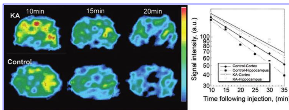
FIG. 15. EPRI of the rat brain. Left: The dynamic pattern of selected transversal EPR images of the rat head 5 mm posterior to the bregma in the KA-treated and control groups at different times after injection of nitroxyl radicals (MC-PROXYL). Right: Pharmacokinetic curves for brain regions. The cortical half-lives of MC-PROXYL in the control and KA groups were 18.0 \pm 1.2 and 19.2 \pm 0.7 min, respectively, whereas the hippocampal half-lives of MC-PROXYL in the control and KA groups were 10.4 \pm 0.8 and 15.9 \pm 0.7 min, respectively. [Adapted from Yokoyama et al. (190).] KA, kainic acid. Color images are available online.
