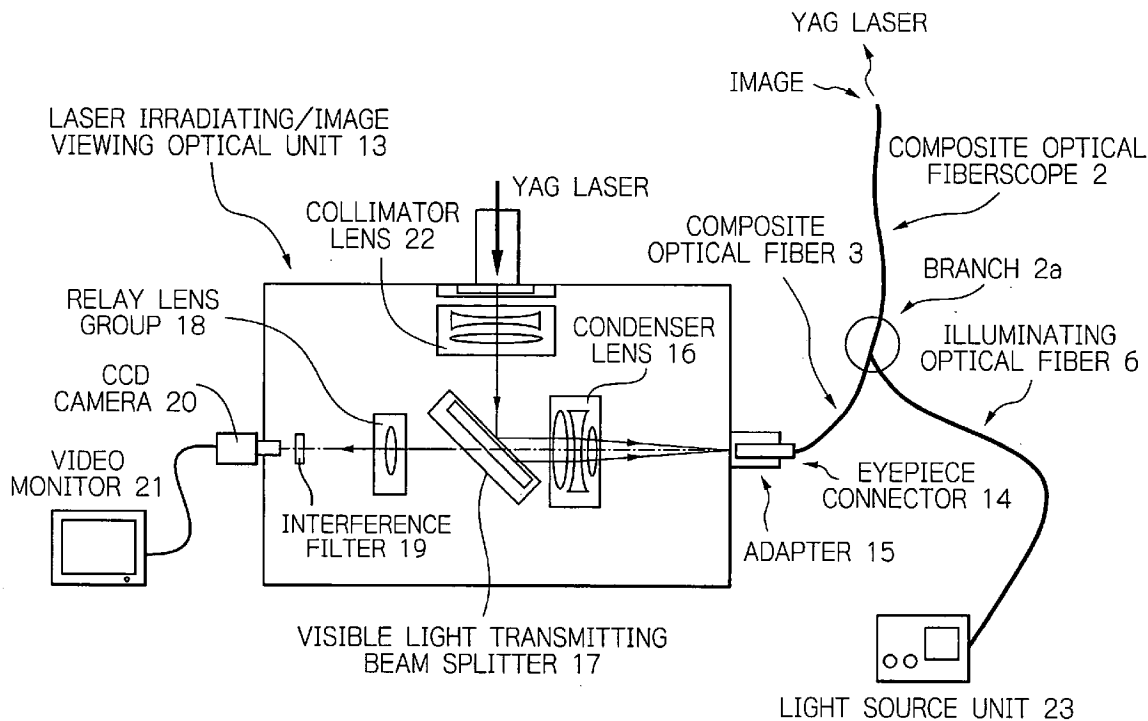
OPTICAL SYSTEM ENABLING IMAGE VIEWING AND LASER LIGHT IRRADIATION
