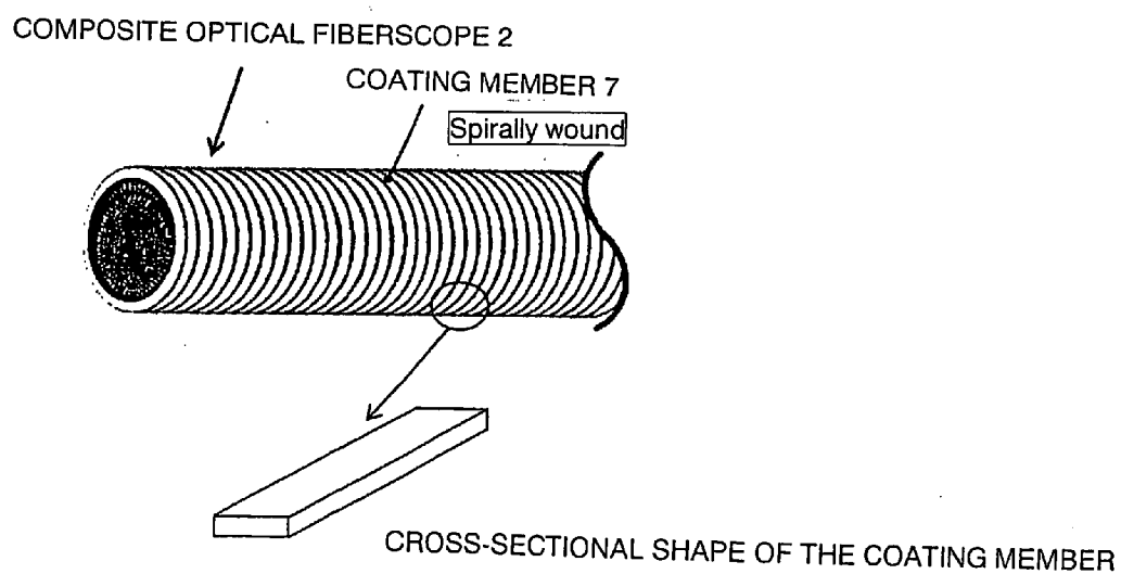
Fig.4 Shape of the coating member
