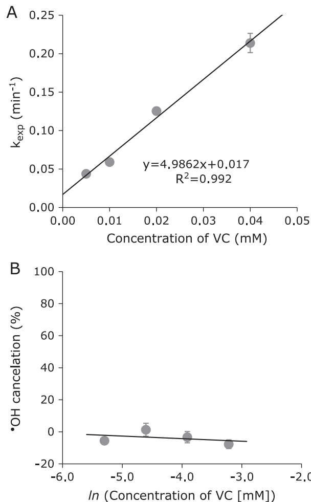
Fig. 3. Assessing antioxidative ability of VC. (A) Estimating second order rate constant, k_{2\text{nd}} , of reducing DMPO-OH by VC. (B) Estimating \text{IC}_{50} value of \cdot\text{OH} -scavenging ability of VC, while no \cdot\text{OH} -scavenging ability was obtained for VC at this concentration level.
